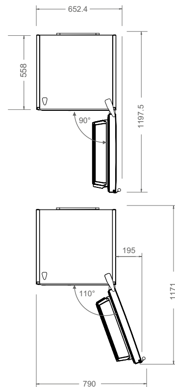
TOP VIEW
