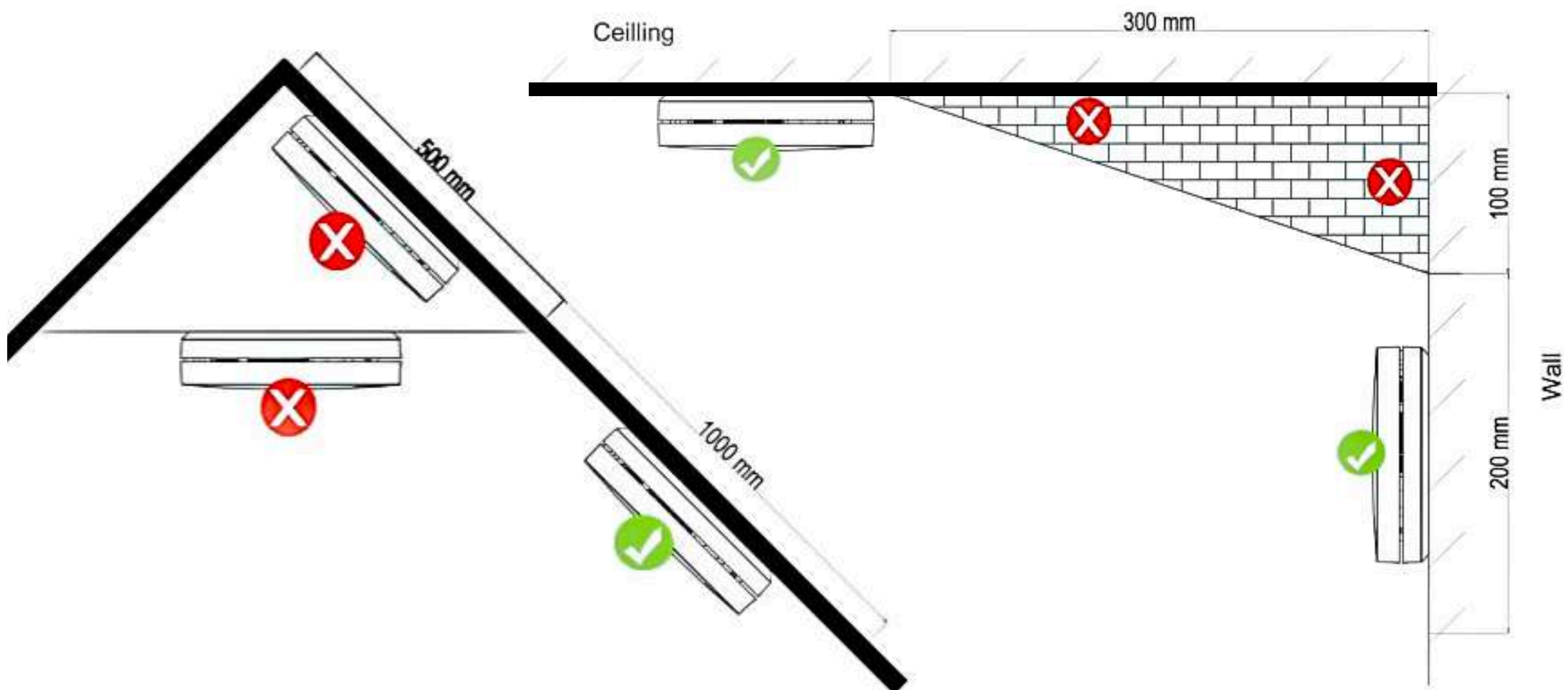
Figure 4: Recommended mounting locations
