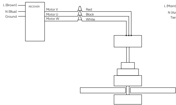
SUPPLY CIRCUIT
