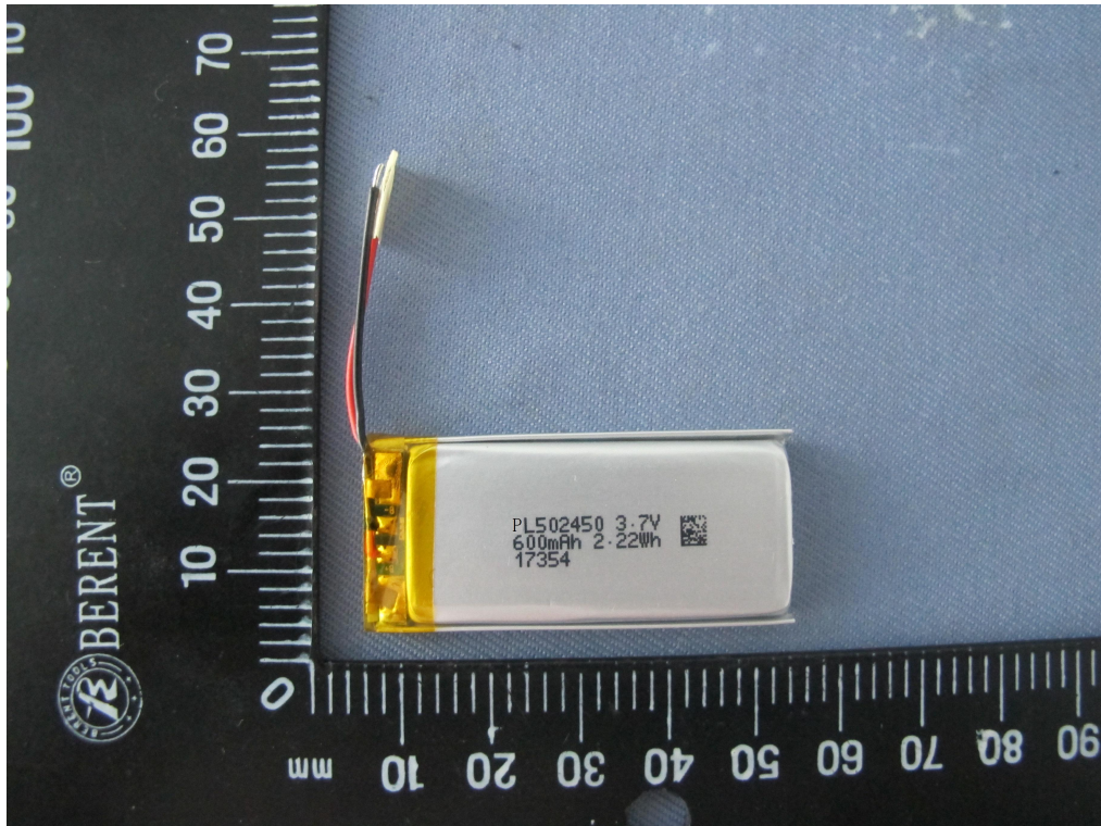
Figure 1 Overall view I of battery (电池图I)
