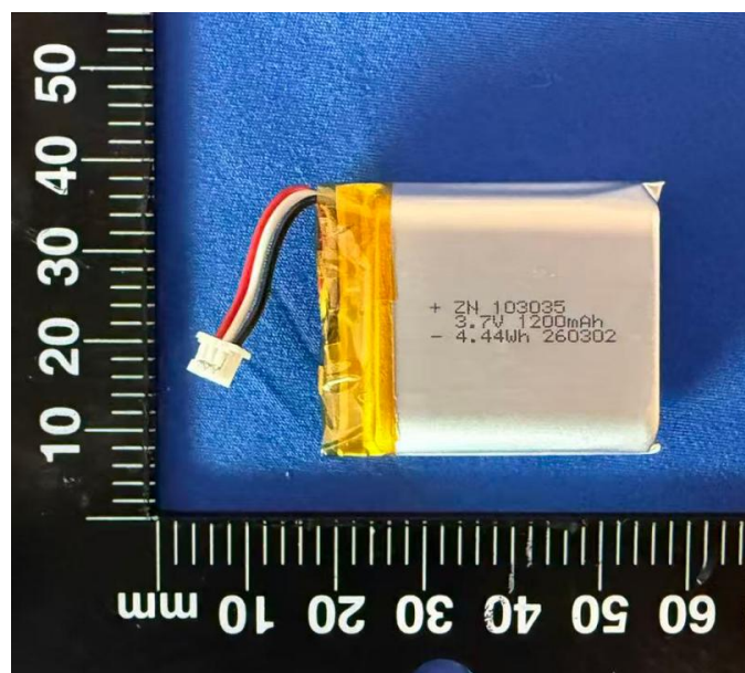
Fig. 2 – Back view of Battery 表2-电池反面视图
