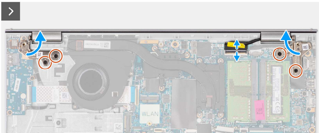
4x M2.5x5
