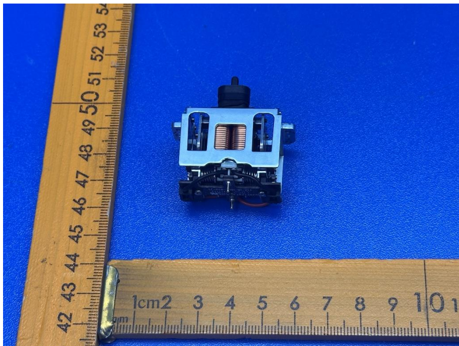
Figure 38. DC motor view (Model LFESP3)
