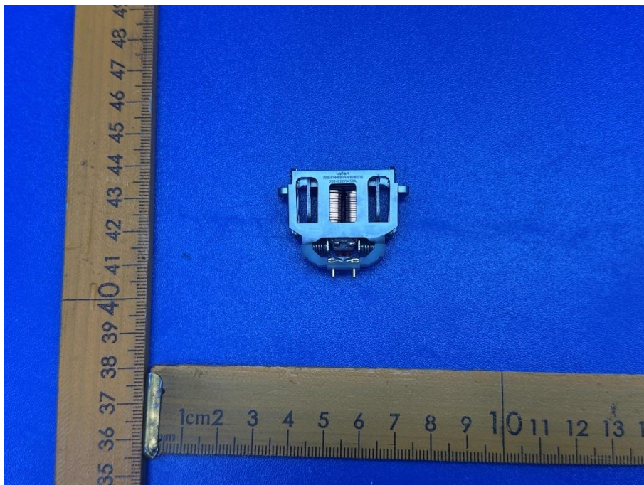
Figure 10. DC motor view (Model LFEST1)
