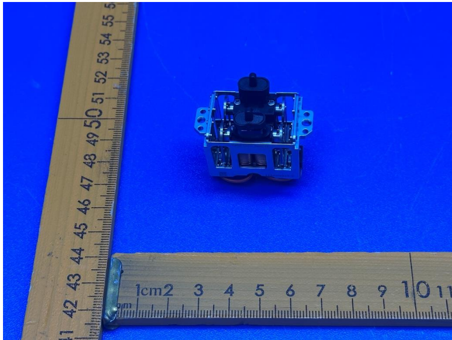
Figure 37. DC motor view (Model LFESP3)
