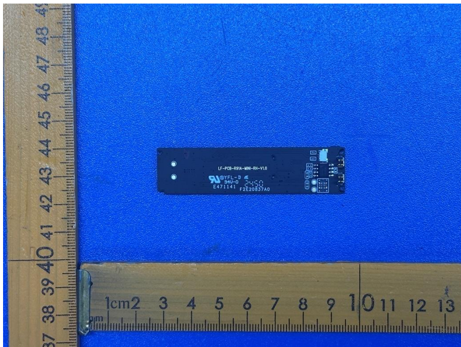
Figure 16. Main PCB view (Model LFEST1)
