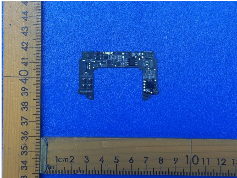
Figure 39. Main PCB view (Model LFESP3)
