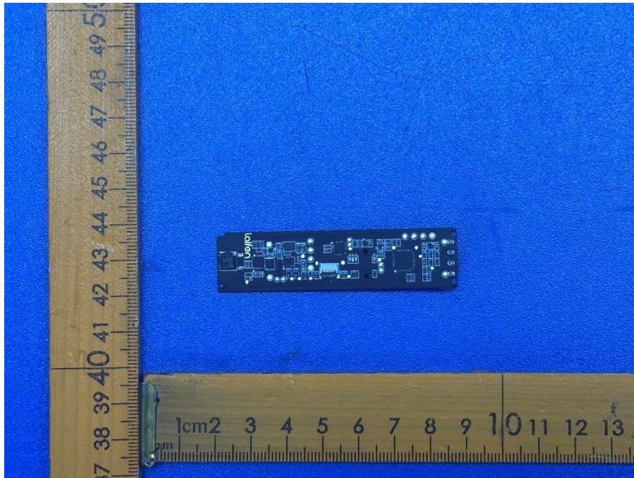
Figure 15. Main PCB view (Model LFEST1)
