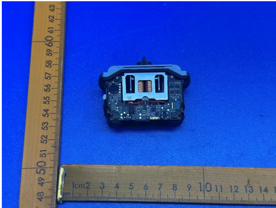
Figure 31. Internal view (Model LFESP3)
