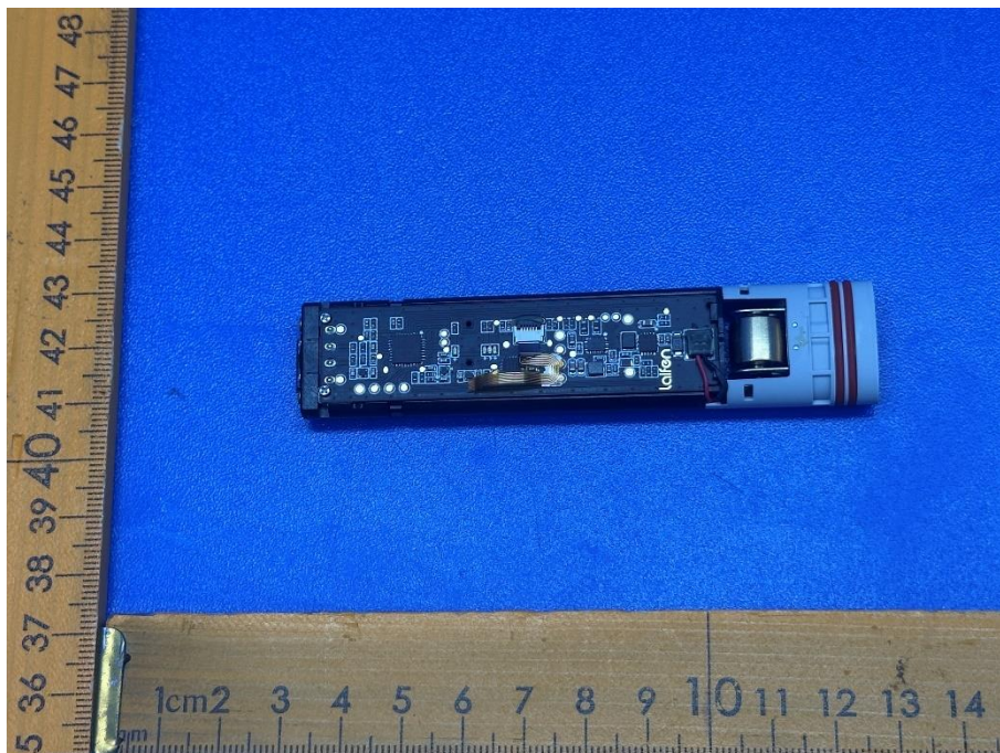
Figure 12. Internal view (Model LFEST1)
