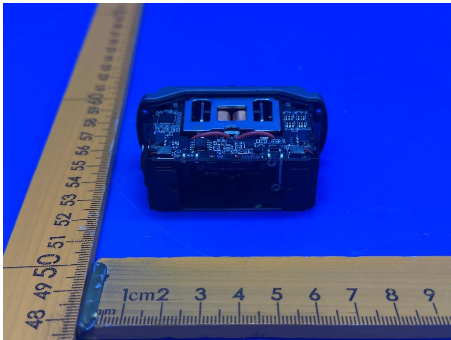
Figure 34. Internal view (Model LFESP3)
