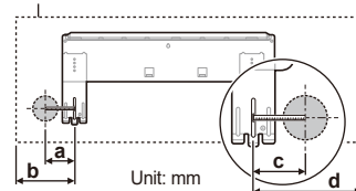
Framework of Indoor Unit
